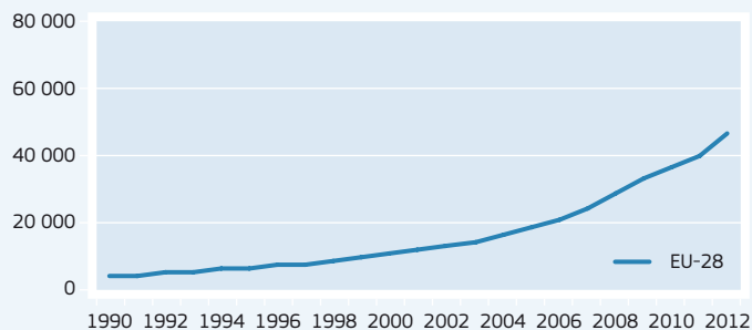
Solar Collectors' Surface – 1990–2012 (1 000 m 2 )
